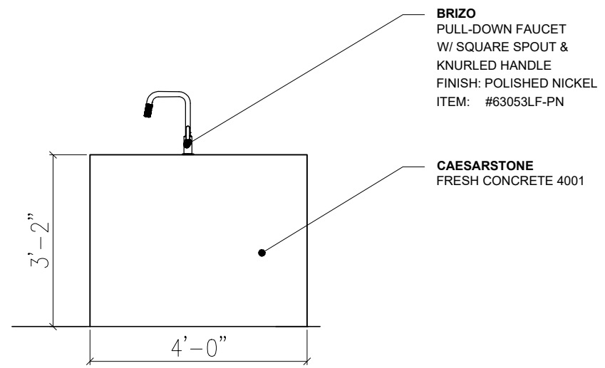
7 KITCHEN ELEVATION S
