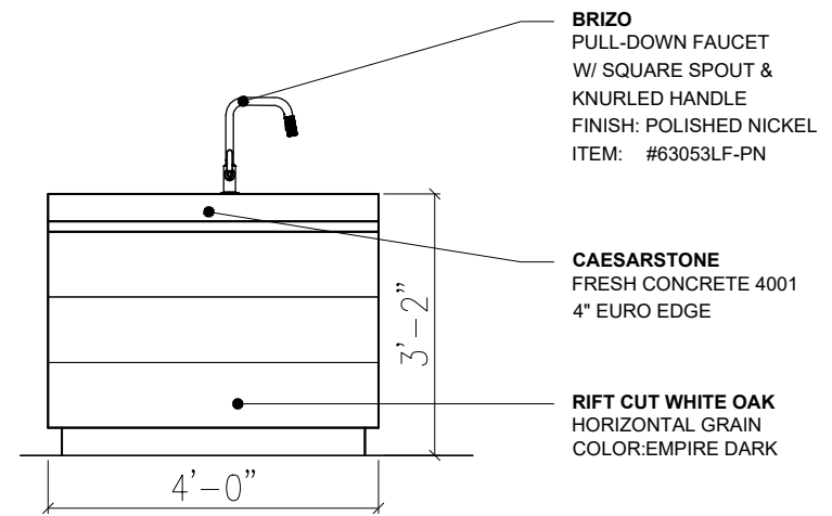
5 KITCHEN ELEVATION N
